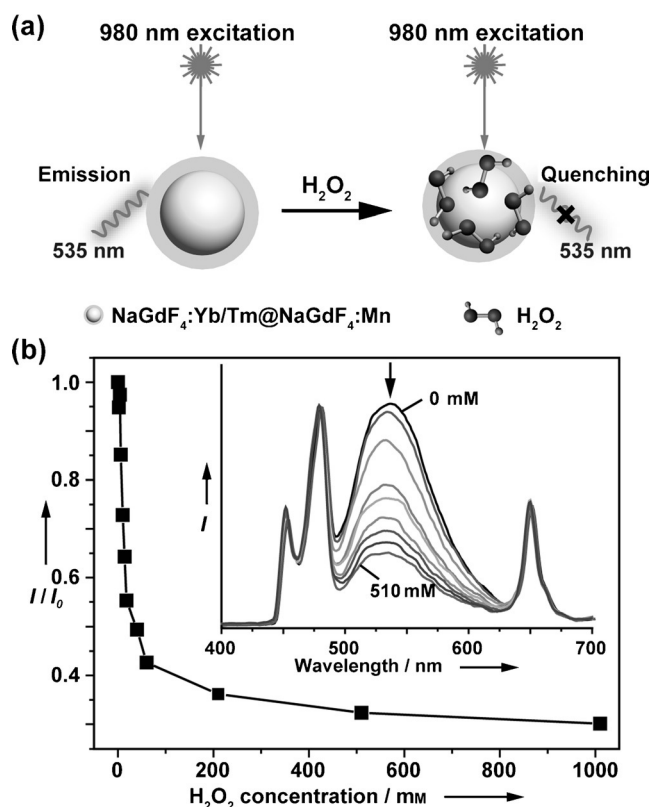
Figure 4. a) \text{H}_2\text{O}_2 sensing by using \text{NaGdF}_4:\text{Yb}/\text{Tm}@\text{NaGdF}_4:\text{Mn} nanoparticles. In the presence of \text{H}_2\text{O}_2 molecules, the upconverted emission of \text{Mn}^{2+} from the core-shell nanoparticles at 535 nm can be suppressed by the oxidation of \text{Mn}^{2+} by \text{H}_2\text{O}_2 . b) Emission intensity dependence (as measured by the ratio of I/I_0 at 535 nm) on \text{H}_2\text{O}_2 concentration (0, 2, 6, 10, 14, 40, 60, 210, and 510 mM). The change in the upconversion emission spectrum as a function of \text{H}_2\text{O}_2 concentration added to the particle solution is shown as inset. The spectra were obtained by irradiating the solution with a pulsed OPO laser to minimize the thermal heating effect. Note that the core-shell nanoparticles used in this study were pretreated with concentrated HCl to afford ligand-free particles readily dispersible in aqueous solutions.
