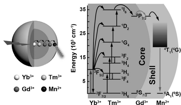
Figure 1. Illustration (left) and proposed energy transfer mechanism (right) of the \text{Mn}^{2+} -activated core-shell upconversion nanoparticles. Note that the core and shell regions are featured in different shades, and the energy transfer occurs through the \text{Yb} \rightarrow \text{Tm} \rightarrow \text{Gd} \rightarrow \text{Mn} pathway in the core-shell nanoparticles upon 980 nm excitation.
