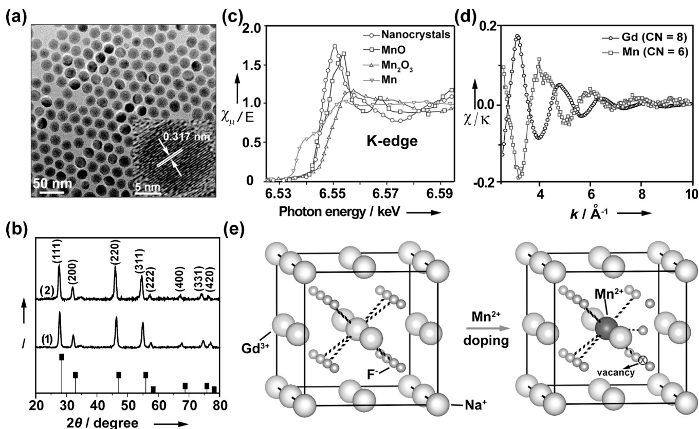
Figure 2. Structural characterization of the \text{NaGdF}_4\text{:Yb/Tm@NaGdF}_4\text{:Mn} nanoparticles. a) TEM image of the as-synthesized nanoparticles (inset: HRTEM image of a single-crystalline nanoparticle). b) XRD patterns of the as-synthesized 1) \text{NaGdF}_4\text{:Yb/Tm@NaGdF}_4 and 2) \text{NaGdF}_4\text{:Yb/Tm@NaGdF}_4\text{:Mn} nanoparticles, as indexed against the standard diffraction patterns of cubic \text{NaYbF}_4 crystals (Joint Committee on Powder Diffraction Standards file number 27-1426). c) Mn K-edge XANES spectra recorded for \text{NaGdF}_4\text{:Yb/Tm@NaGdF}_4\text{:Mn} nanoparticles, \text{MnO} , \text{Mn}_2\text{O}_3 , and Mn metal, respectively. d) Experimental Gd \text{L}_{3\text{-edge}} and Mn K-edge EXAFS in k -space for \text{NaGdF}_4\text{:Yb/Tm@NaGdF}_4\text{:Mn} nanoparticles. e) Schematic presentation of \text{NaGdF}_4 crystal structures without and with \text{Mn}^{2+} dopant ions. Note that upon substitution of \text{Gd}^{3+} with \text{Mn}^{2+} ions, \text{F}^- vacancies may be introduced for maintaining the charge neutrality, thus resulting in a decrease in the coordination number of the \text{Mn}^{2+} ions.
