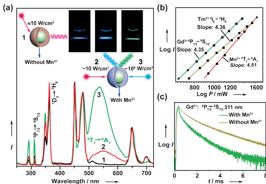
Figure 3. a) Upconversion emission profiles of 1) \text{NaGdF}_4\text{:Yb/Tm@NaGdF}_4 and 2) \text{NaGdF}_4\text{:Yb/Tm@NaGdF}_4\text{:Mn} nanoparticles recorded at room temperature under 980 nm CW excitation as well as 3) \text{NaGdF}_4\text{:Yb/Tm@NaGdF}_4\text{:Mn} nanoparticles irradiated with a pulsed OPO laser at a power density of 10^8 \text{ W cm}^{-2} . The corresponding luminescence photos taken from cyclohexane solutions of the nanoparticles are inset. b) Log-log plots of the upconversion emission against the excitation power at 980 nm for ^6\text{P}_{7/2} \rightarrow ^8\text{S}_{7/2} transition of \text{Gd}^{3+} , ^1\text{I}_6 \rightarrow ^3\text{H}_6 transition of \text{Tm}^{3+} , and ^4\text{T}_1 \rightarrow ^6\text{A}_1 transition of \text{Mn}^{2+} . c) A comparison of upconversion lifetimes of \text{Gd}^{3+} in \text{NaGdF}_4\text{:Yb/Tm@NaGdF}_4\text{:Mn} and \text{NaGdF}_4\text{:Yb/Tm@NaGdF}_4 nanoparticles. Note that the core-shell nanoparticles used in the time-decay measurement were pretreated with concentrated HCl to remove the surface oleate ligands that may quench the upconversion emission at around 300 nm.
